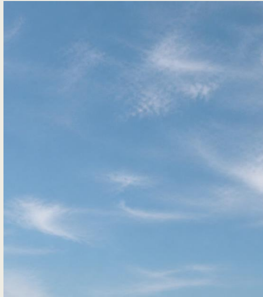
Clear
