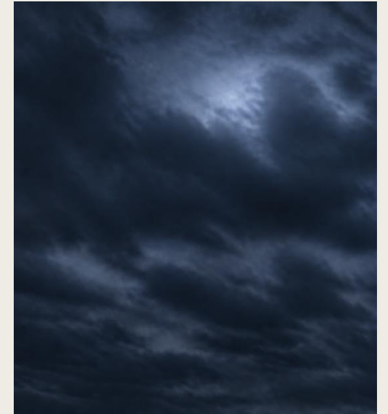
Storm
