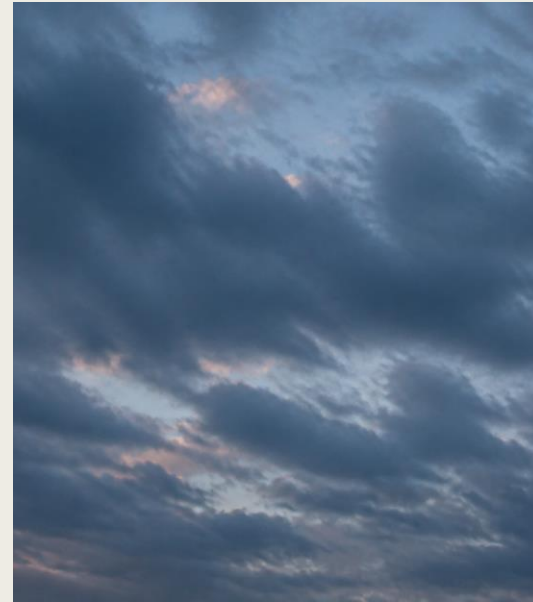
Cloudy
